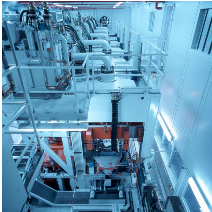
View from above of the Läßle presses. The hydraulic power units are installed above the tool magazines.
