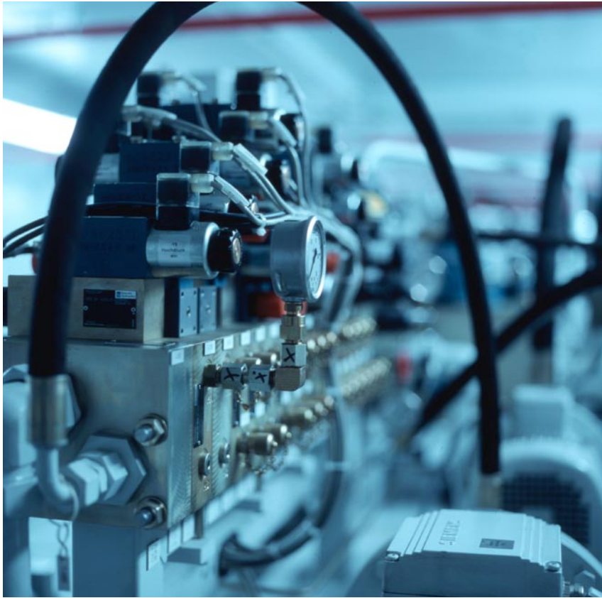
View of the IH20 control for the press auxiliary movements.
